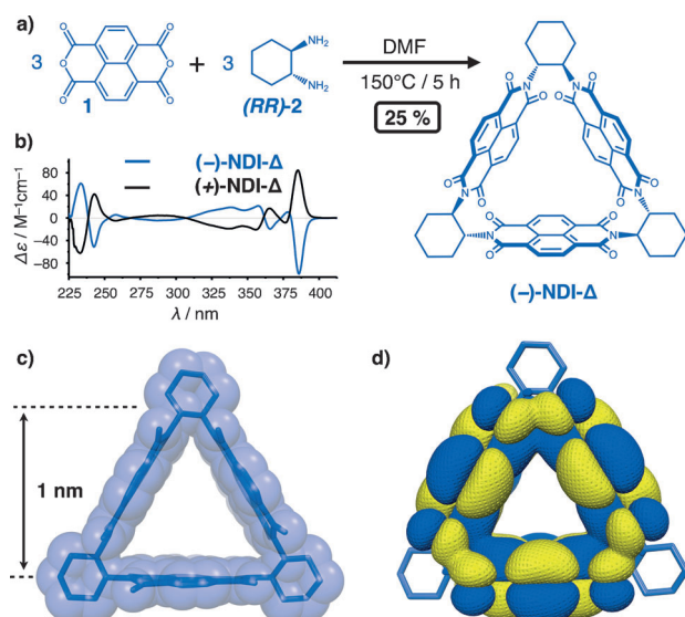
Figure 1. a) Stereospecific synthesis of the rigid triangular molecular prism (-) -NDI- \Delta from (RR) - 2 . The enantiomer (+) -NDI- \Delta was prepared in a similar yield from (SS) - 2 , following the same procedure as that used to prepare the (-) -enantiomer. b) CD spectra of (-) - and (+) -NDI- \Delta recorded at 298 K in \text{CH}_2\text{Cl}_2 solutions. c) Tubular representation of the single-crystal X-ray structure of (-) -NDI- \Delta with the corresponding space-filling representation superimposed upon it in a semi-transparent fashion. d) Graphical representations of the DFT-calculated (B3LYP/6-31G**) lowest unoccupied molecular orbital (LUMO) of (-) -NDI- \Delta . Orbital isosurfaces are illustrated at 0.004 electrons \text{Bohr}^{-3} .
