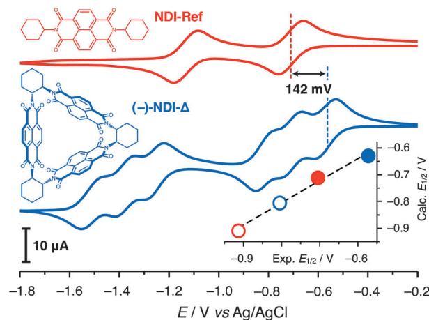
Figure 2. Cyclic voltammograms (CVs) of a reference NDI compound (NDI-Ref) with cyclohexyl substituents (red curve) and (-) -NDI- \Delta (blue curve) recorded (scan rate 50 \text{ mVs}^{-1} ) using a glassy carbon electrode. All of the experiments were performed at 298 K in argon-purged \text{CH}_2\text{Cl}_2 solutions (0.5 mm) with 0.1 \text{ M } [\text{Bu}_4\text{N}][\text{PF}_6] as the supporting electrolyte. The inset shows the correlation between the DFT-calculated and the experimental half-wave potentials ( E_{1/2} vs. Ag/AgCl) for the first reductions of (-) -NDI- \Delta (blue ●), NDI-Ref (red ●), and the corresponding compounds (○) with all of the NDI groups replaced with pyromellitic diimide (PMI) functional groups. A linear fit to the data ( y = 1.20x + 0.16 \text{ V} ) gave a coefficient of correlation ( R^2 ) of 0.99.
